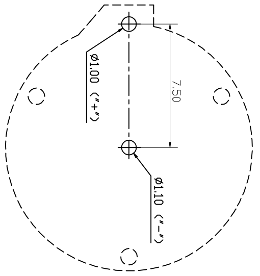
PCB LAYOUT
